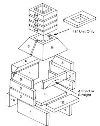
4 Chimney Extensions, Hearth • Risers 18"H • Firebrick
