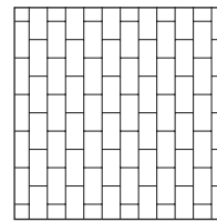
Running Bond Head On
